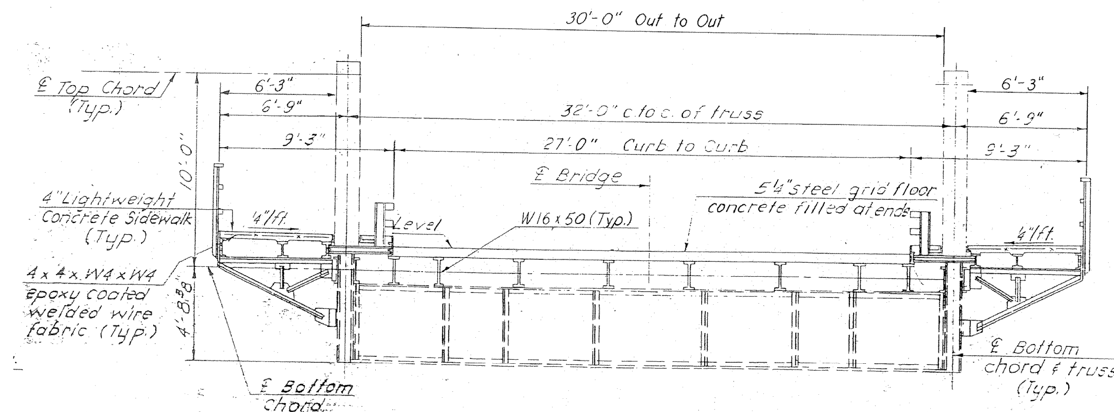
KINGSLAND AVENUE BRIDGE EXISTING BRIDGE SECTION
