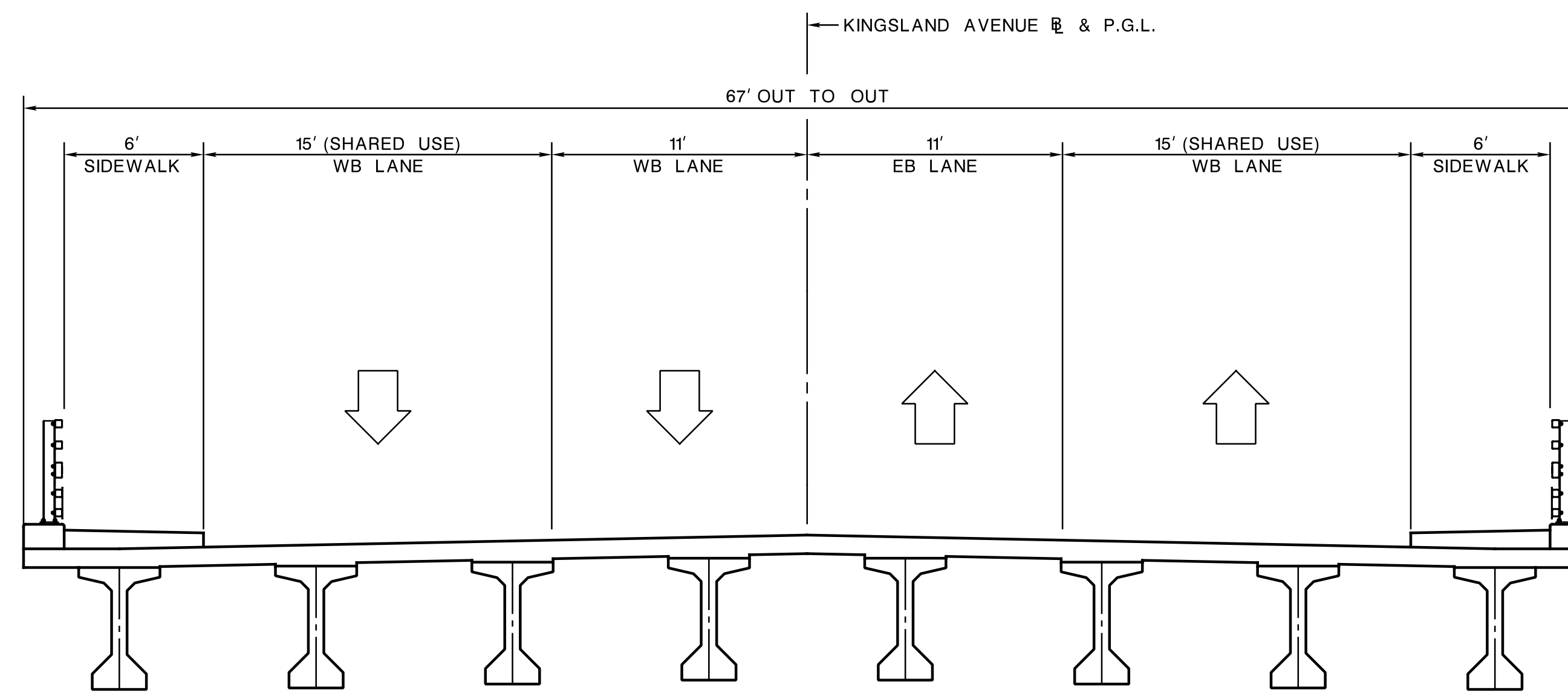
KINGSLAND AVENUE BRIDGE PROPOSED 4-LANE BRIDGE SECTION
