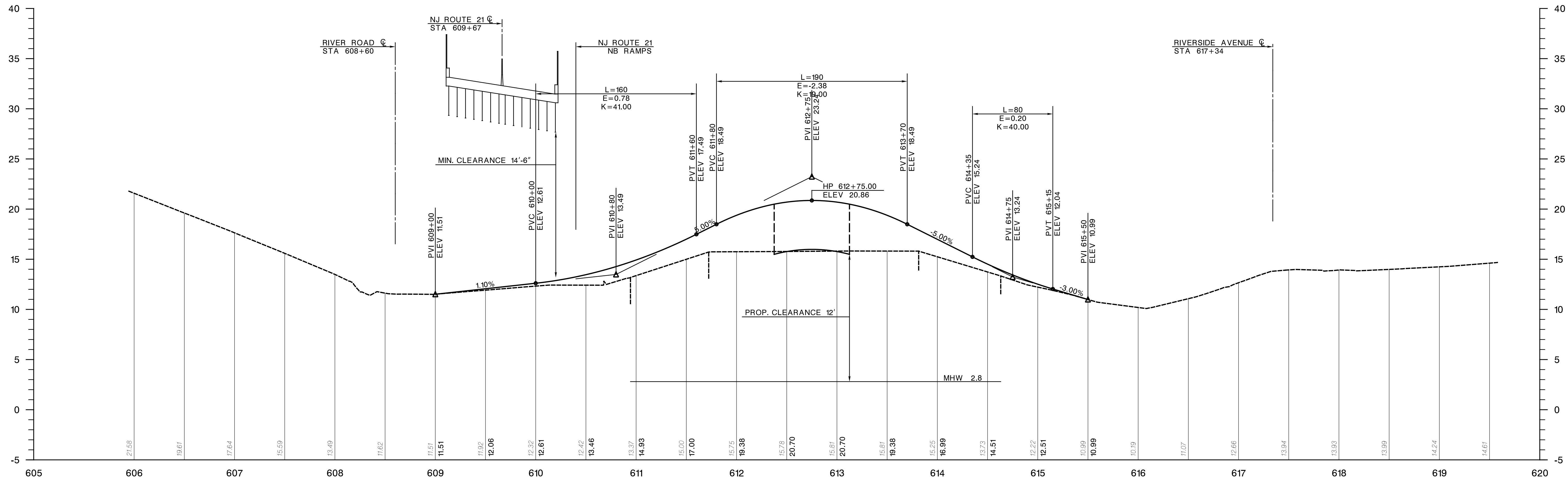
KINGSLAND AVENUE / PARK AVENUE ALTERNATIVE PROFILE (12' ABOVE MHW) - 75' WIDE CHANNEL
