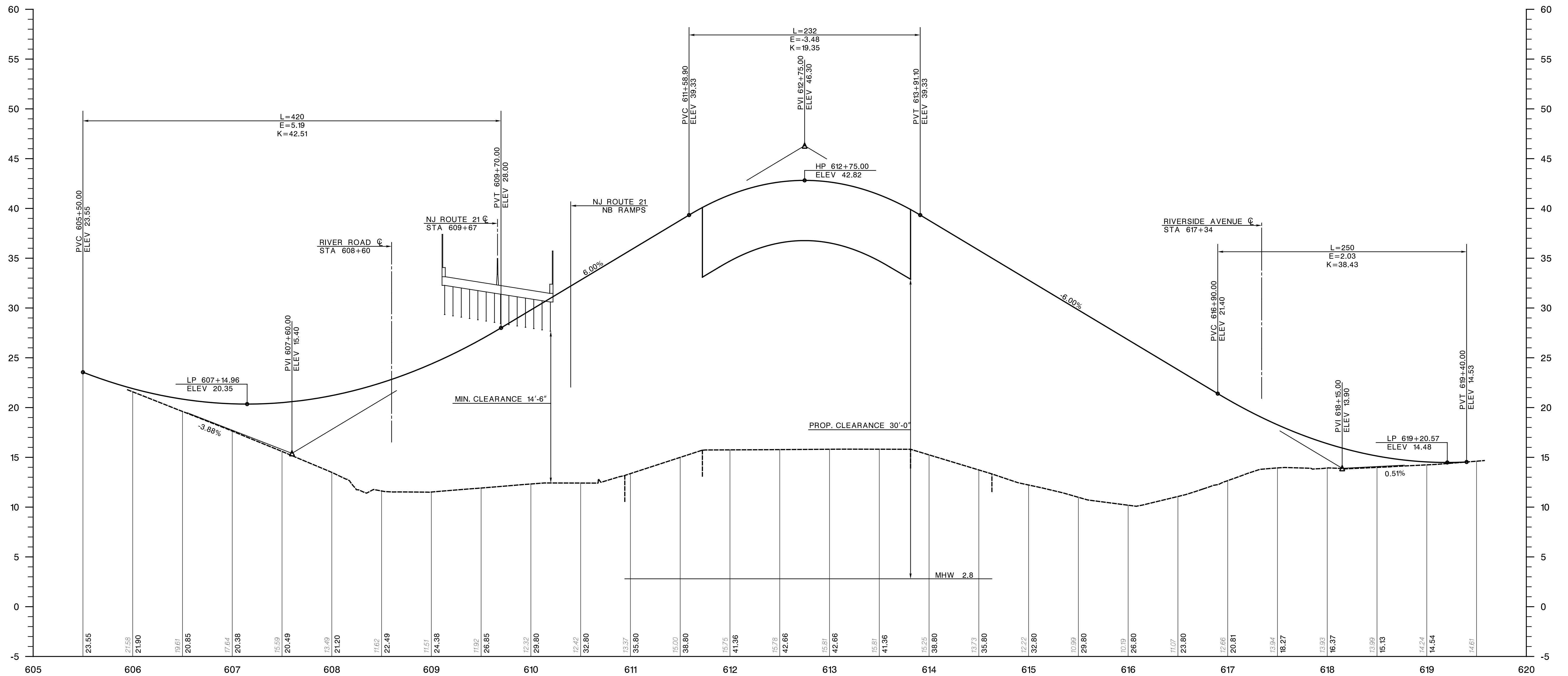
KINGSLAND AVENUE / PARK AVENUE ALTERNATIVE PROFILE (30' ABOVE MHW)
